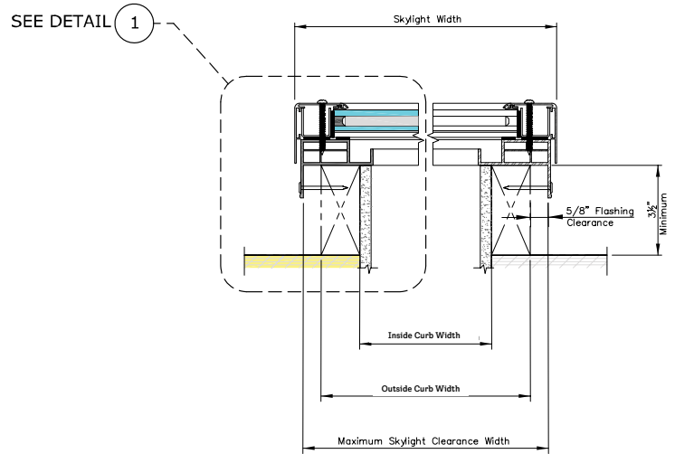
HORIZONTAL CROSS SECTION
