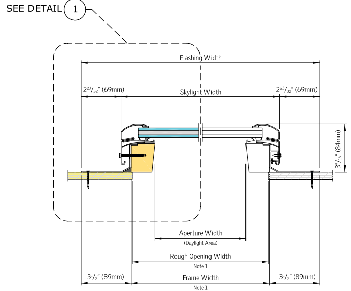
HORIZONTAL CROSS SECTION
